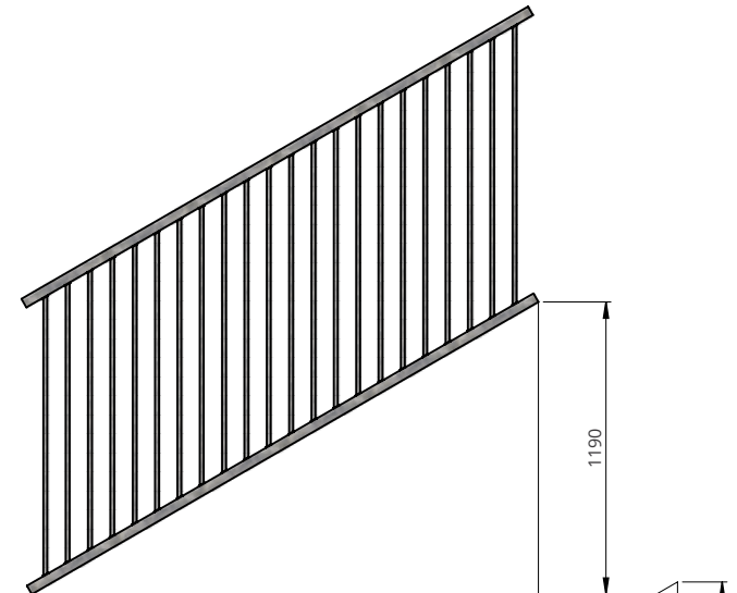
30 DEGREE RAKE
