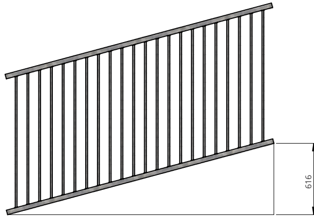
15 DEGREE RAKE
